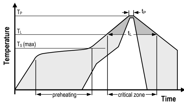
Figure 5: Soldering profile according to JEDEC standard. T_P \leq 260^\circ\text{C} and t_P < 40\text{sec} for Pb-free assembly. T_L < 220^\circ\text{C} and t_C < 150\text{sec} . Ramp-up/down speeds shall be < 5^\circ\text{C}/\text{sec} .
