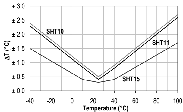
Figure 3: Maximal T-tolerance per sensor type.
